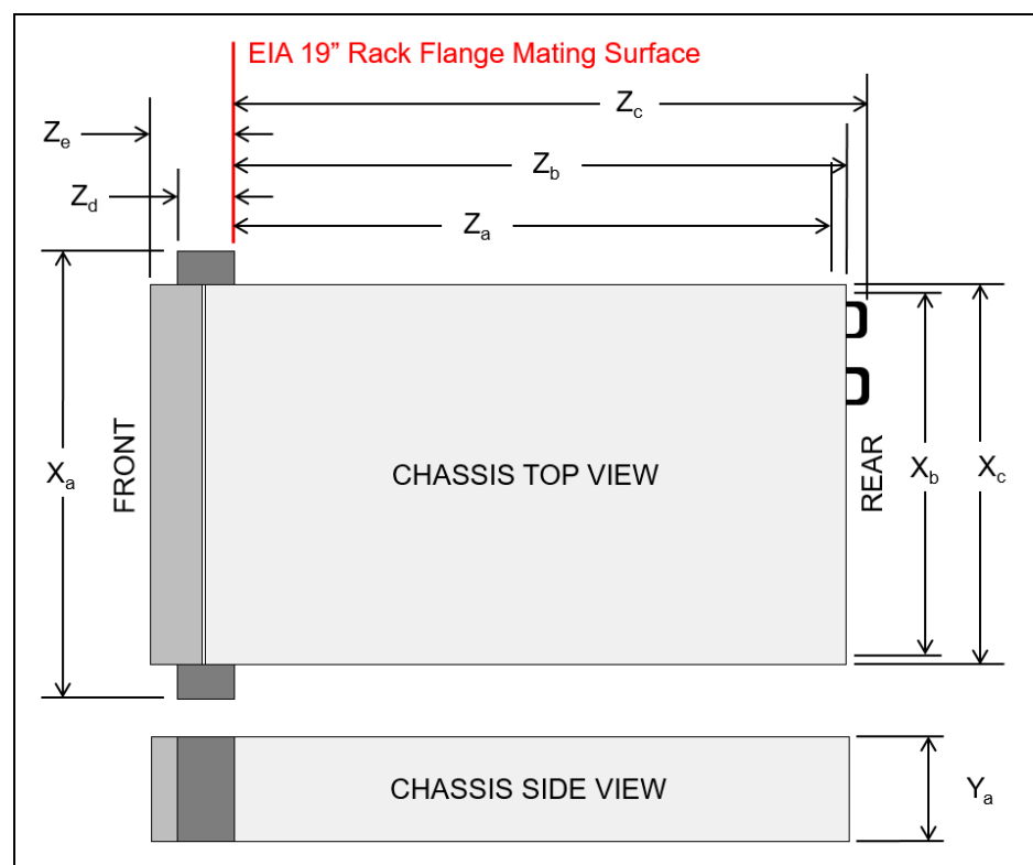
Figure 12. Server dimensions
