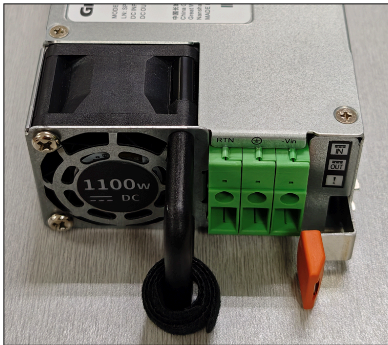
Figure 21. Connector on the ThinkSystem 1100W -48V DC Hot-Swap Gen2 Power Supply v2 (4P57A89415)
