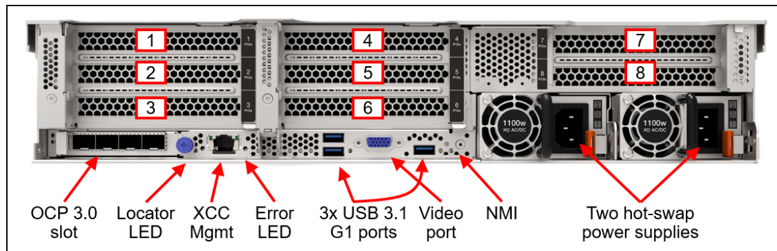
Figure 4. Rear view of the ThinkSystem SR650 V3 (configuration with eight PCIe slots)
